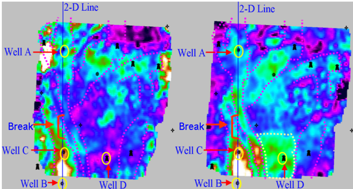
Figure 6a: AVO Fluid Factor, Standard Stack
