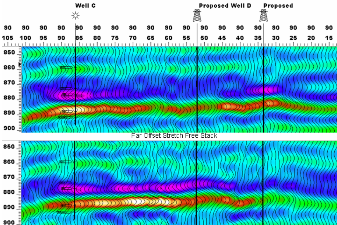
Figure 7: Comparison of East West Lines: Well C and Well D (Prospect)
