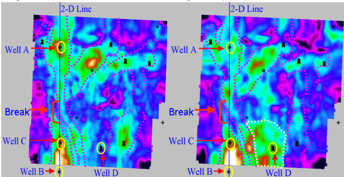
Figure 5a: Amplitudes Far offsets, Standard Stack
