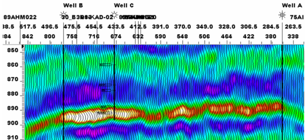
Figure 2: Standard Processing of 2-D Line.
